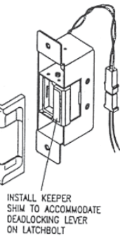
ELECTRIC LOCKSTRIKE
