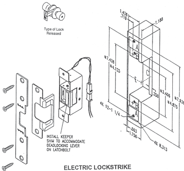
ELECTRIC LOCKSTRIKE
